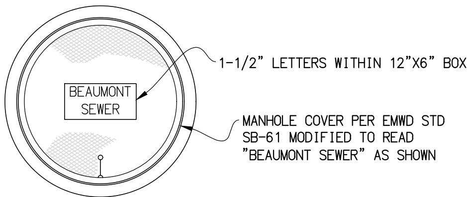
MANHOLE COVER DETAIL
